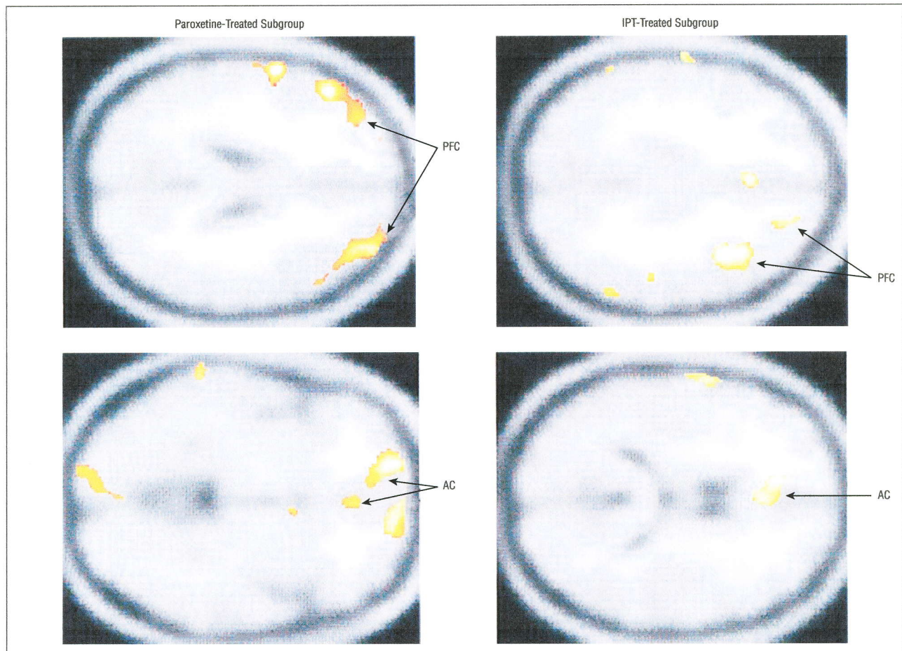
Figure 4. Comparison of relative brain metabolic decreases (Zstatistic, P < .01 ) from baseline to follow-up in major depressive disorder subgroups treated with either paroxetine (n=10) or interpersonal psychotherapy (IPT) (n=14). The paroxetine-treated subgroup showed bilateral prefrontal cortical (PFC) decreases, while the IPT-treated subgroup had changes in right PFC only. Both groups had decreases in left anterior cingulate gyrus (AC).
