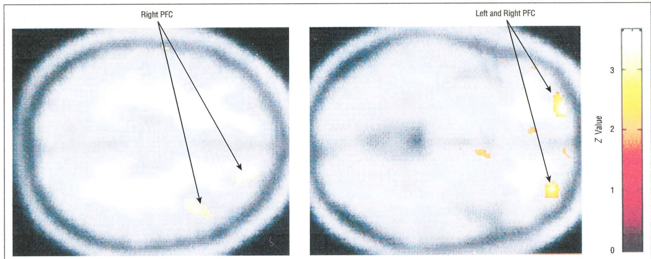
Figure 3. Decreases in relative prefrontal cortical (PFC) metabolism from baseline to follow-up in the total major depressive disorder (MDD) treated group (N=24) (Zstatistic, P < .01 ). Decreases in activity are transposed onto a template magnetic resonance image and are shown in 2 separate planes.
